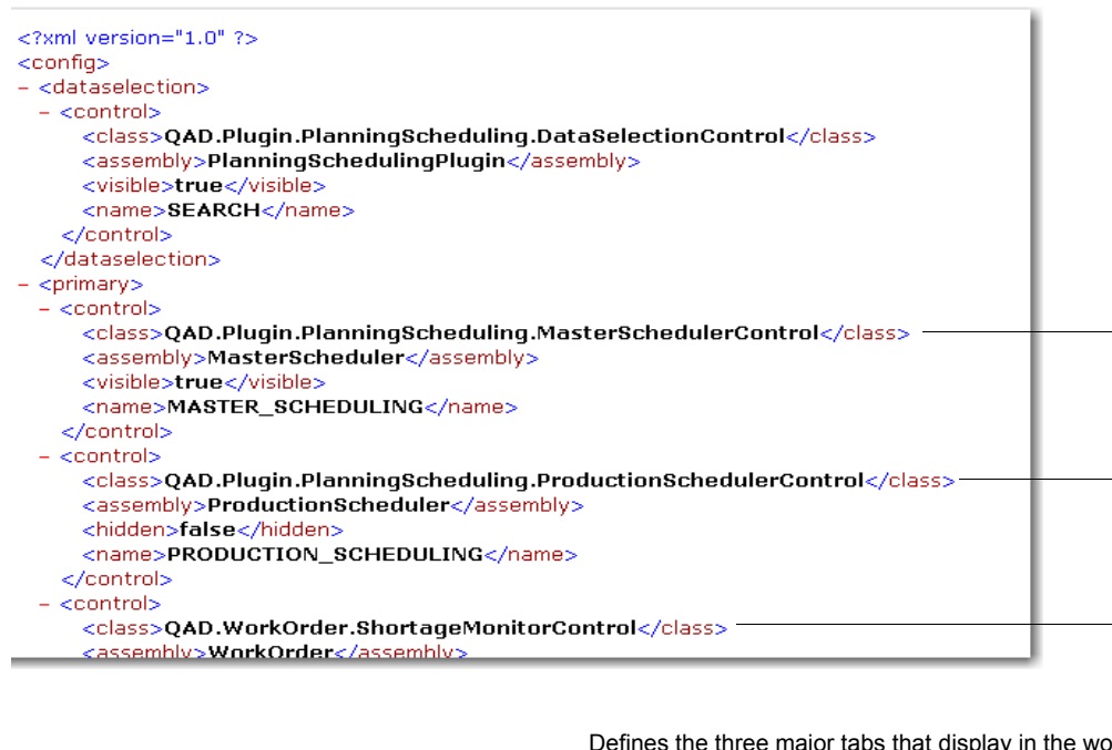
Fig. 4.5 ControlConfig.XML File
