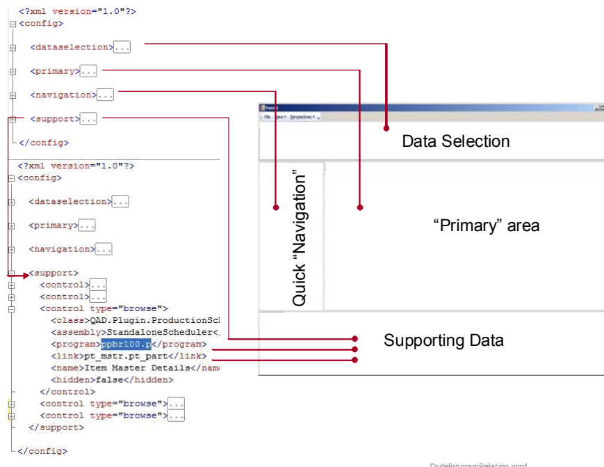
Fig. 4.4 Code-UI Relationship
