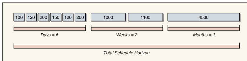
Fig. 4.13 Schedule Bucketing
