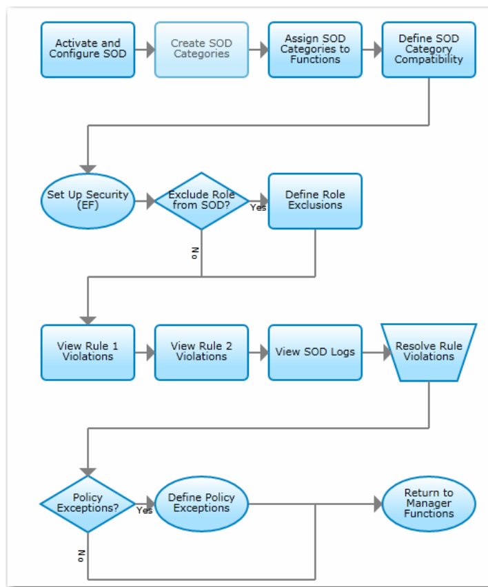
Fig. 7.3 Segregation of Duties Setup Flow
