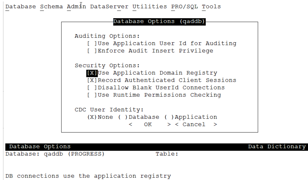
Fig. 10.2 Database Options Settings
