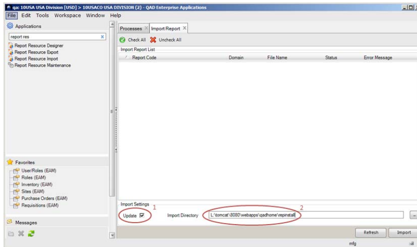
Fig. 20 Import Report
