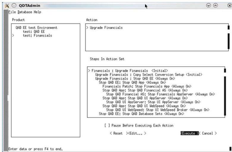
Fig. 10 Backward Compatibility
