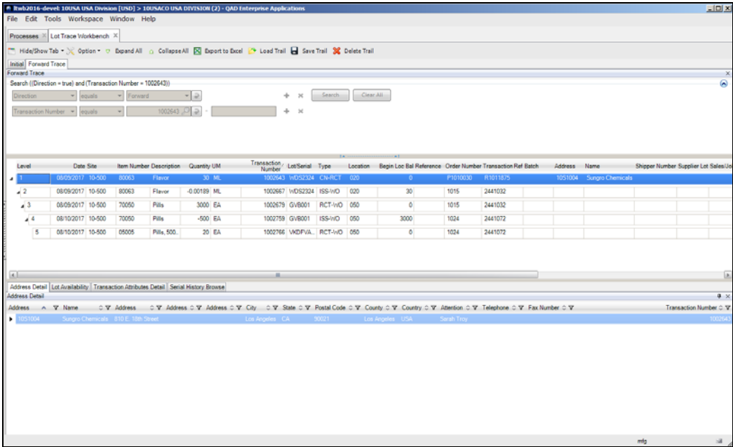
Fig. 8.14 Forward Trace
