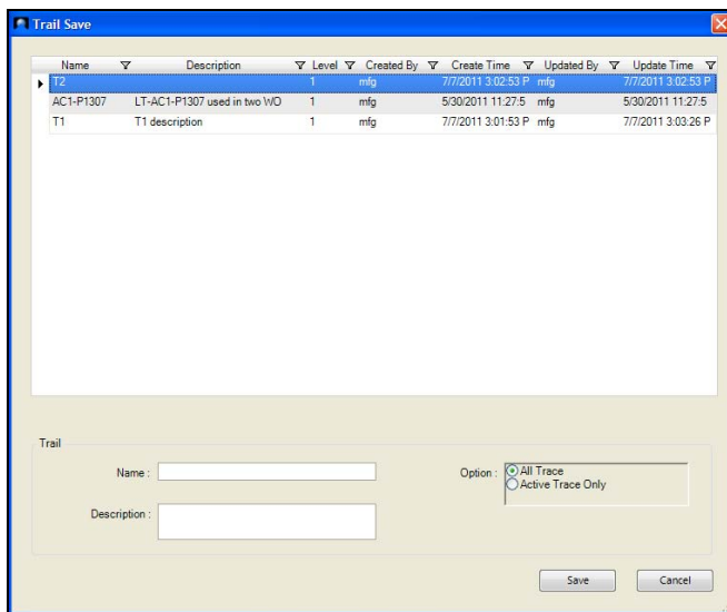
Fig. 8.19 Trail Save
