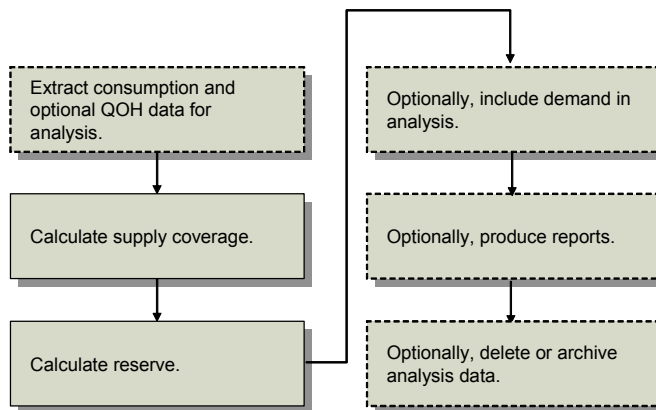
Fig. 8.37 Processing Flow
