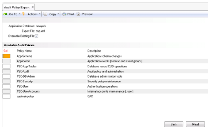
Fig. 11.14 Audit Policy Export (36.12.13.2)
