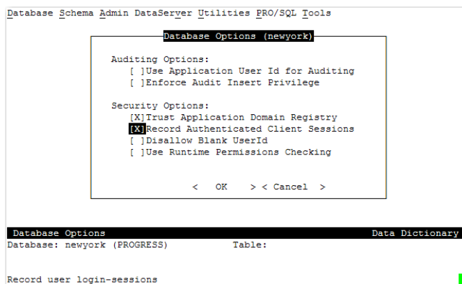
Fig. 11.2 Database Options Settings
