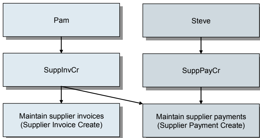
Fig. 9.2 Segregation of Duties Violation
