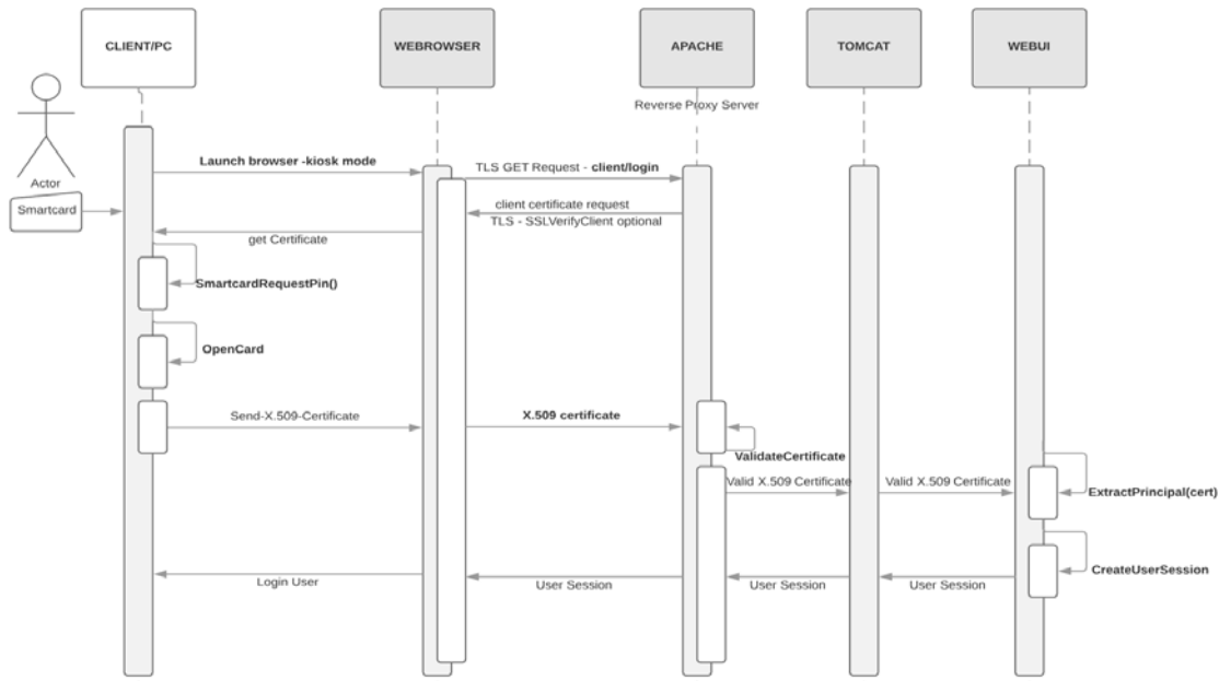
Fig. 5.3 Smart Card Authentication Sequence Diagram
