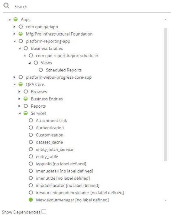
Fig. 7.10 Role Permissions Tree
