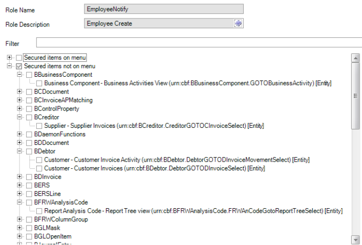
Fig. 6.8 Role Permissions Maintain, Secured Items Not on Menu
