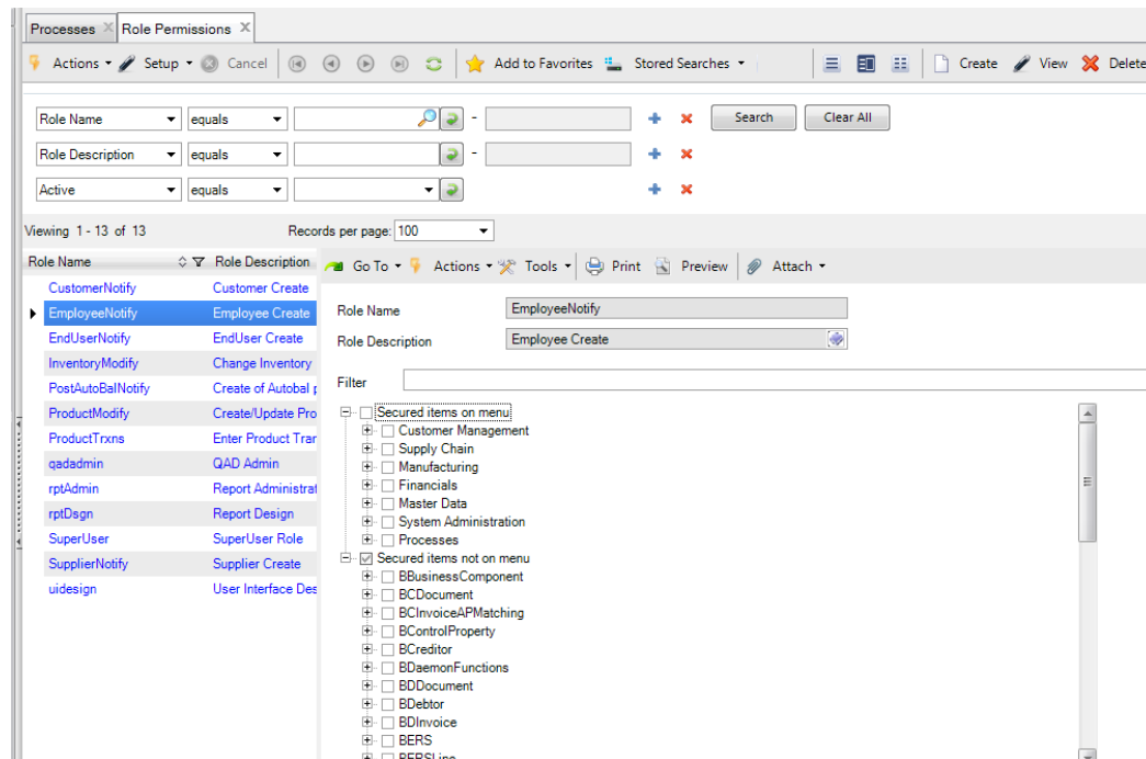
Fig. 6.6 Role Permissions Maintain (36.3.6.5)
