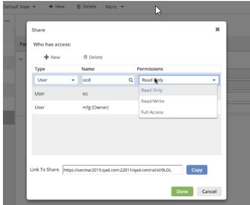
Fig. 7.35 Define Share Access
