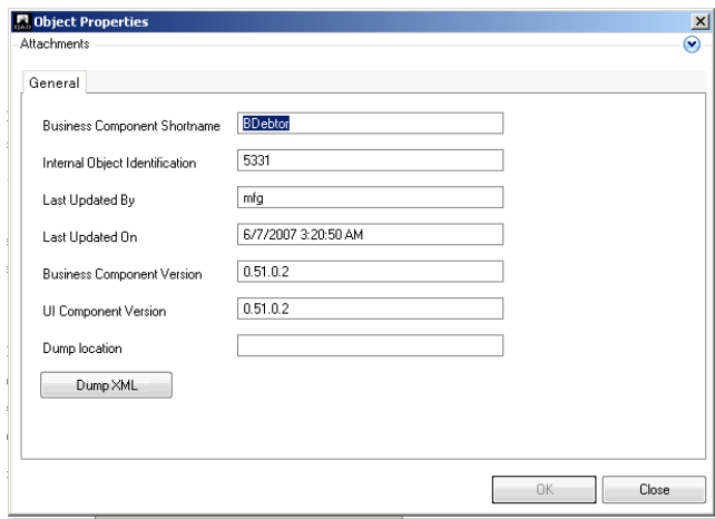
Fig. 3.10 Object Properties
