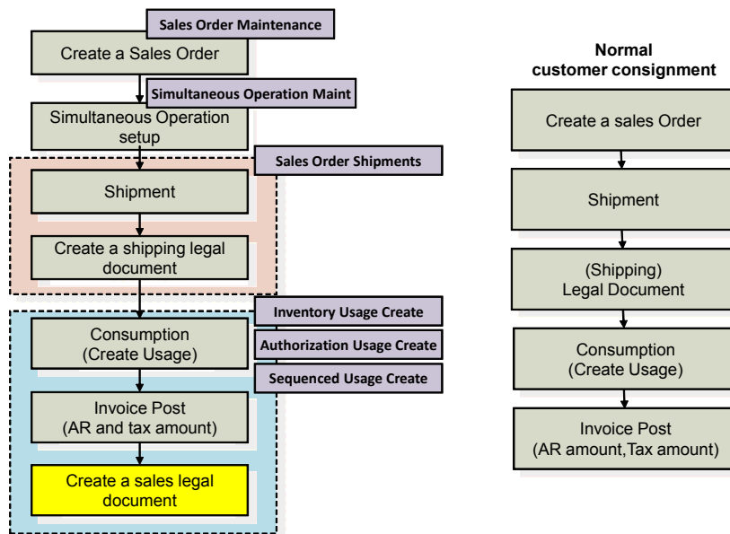
Fig. 12.23 Process Flow of Simultaneous Customer Consignment
