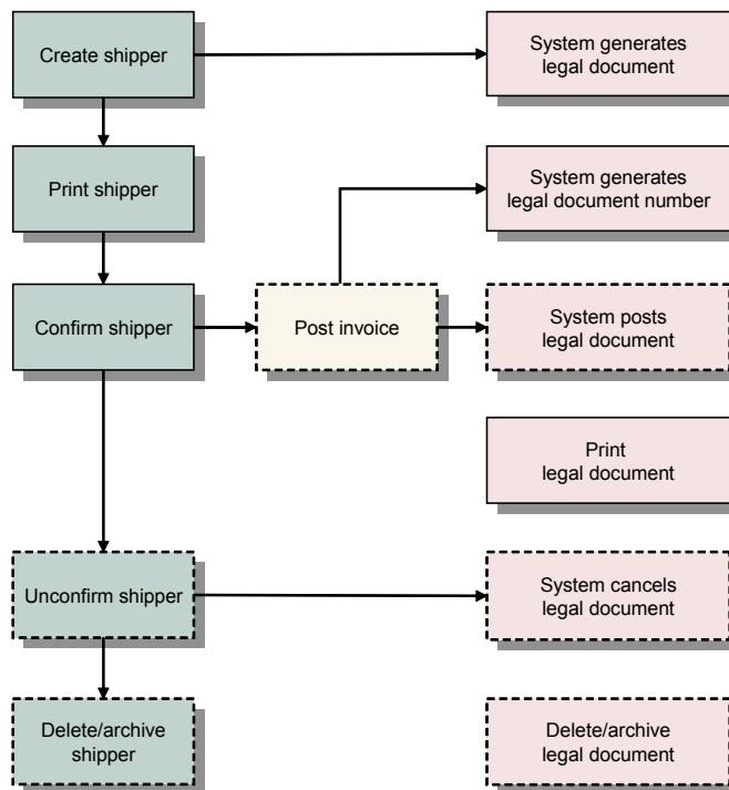
Fig. 12.26 Brazil Legal Document Life Cycle
