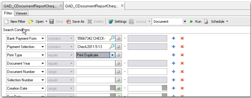
Fig. 6.9 Report Filters
