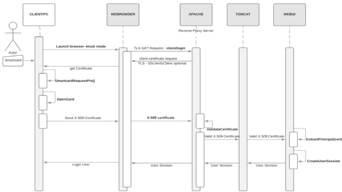
Fig. 5.4 Smart Card Authentication Sequence Diagram
