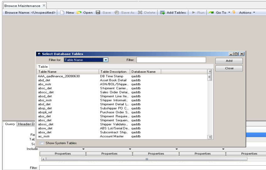
Fig. 4.24 Browse Maintenance
