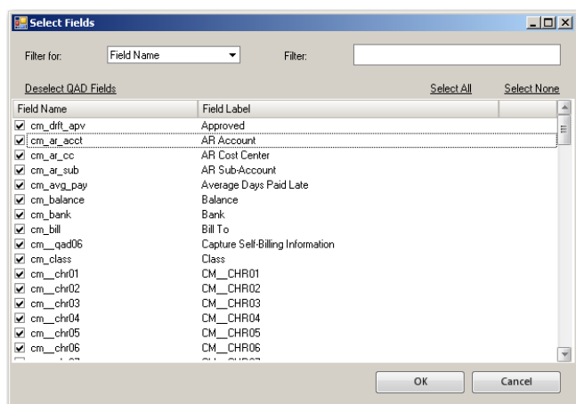
Fig. 4.27 Select Fields
