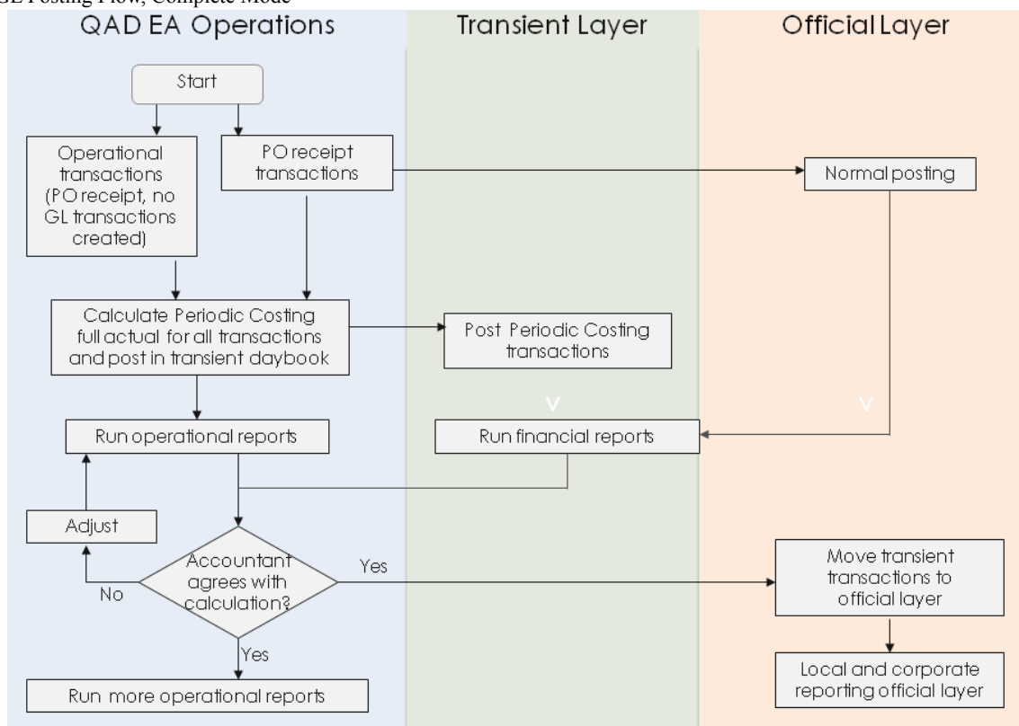
Fig. 1.2 GL Posting Flow, Complete Mode
