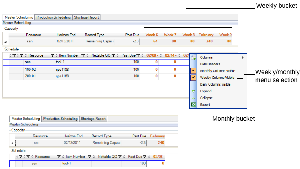
Fig. 2.3 Monthly and Weekly Buckets
