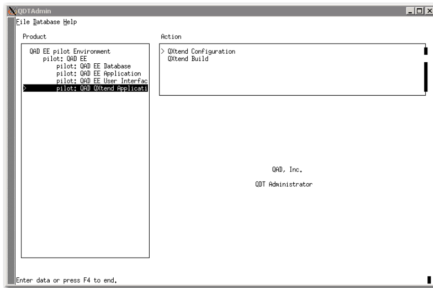
Fig. 4.9 QXtend Configuration
