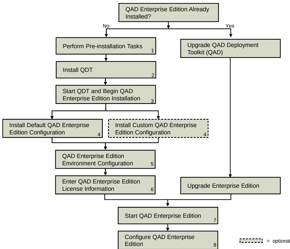
Fig. 1.1 QAD Enterprise Edition Installation Process
