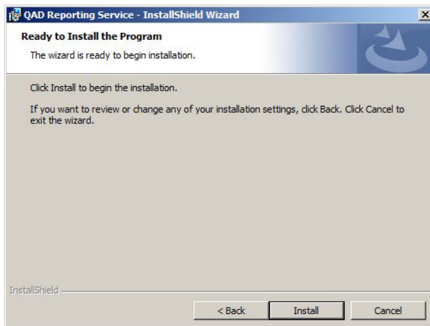
Fig. 6.9 Installation Prompt
