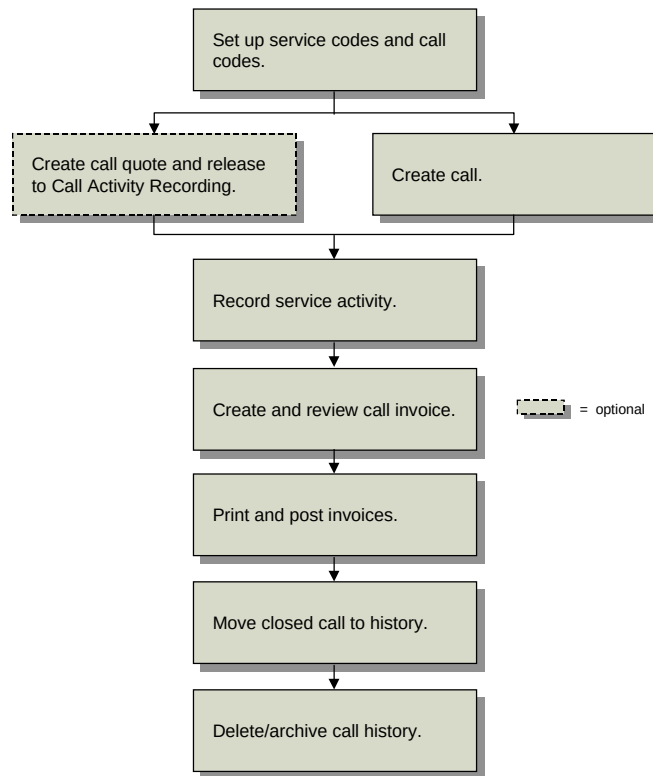
Fig. 14.1 Call Activity Recording in the Call Life Cycle
