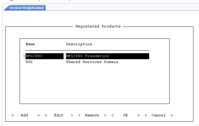
Fig. 8.4 License Registration (36.16.10.1)
