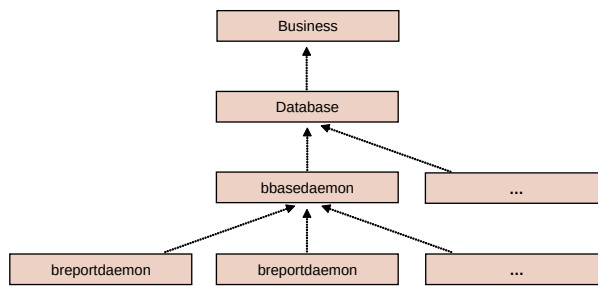
Fig. 10.2 Inheritance Structure
