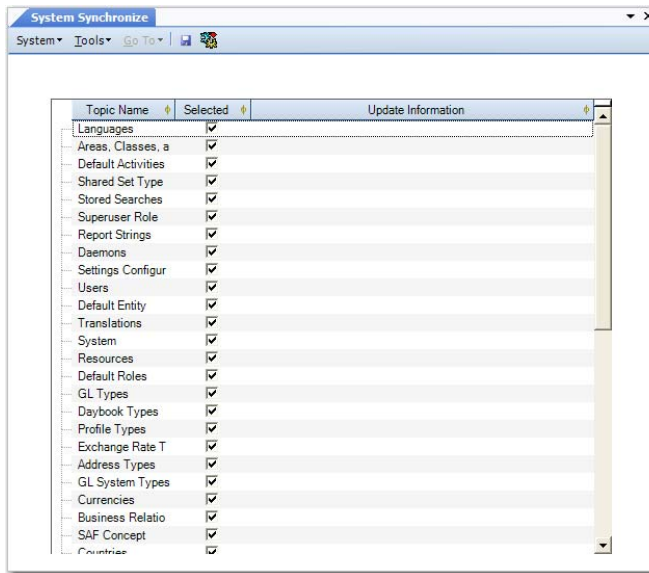
Fig. 6.3 System Synchronize (36.24.3.2)
