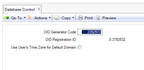
Fig. 6.1 Database Control (36.24.1)
