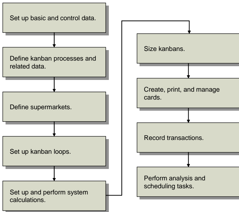
Fig. 3.3 Kanban Workflow
