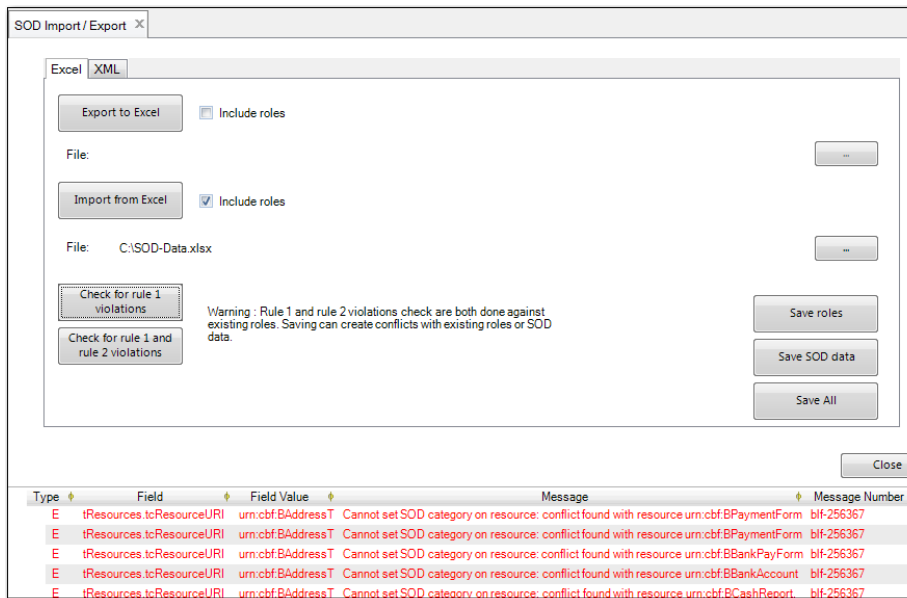
Fig. 5.34 Violation Errors
