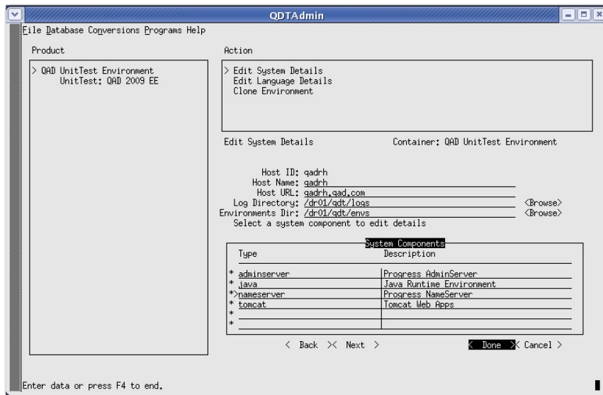
Fig. H.9 Committing Changes
