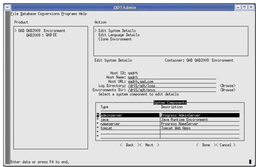
Fig. H.3 System Details List
