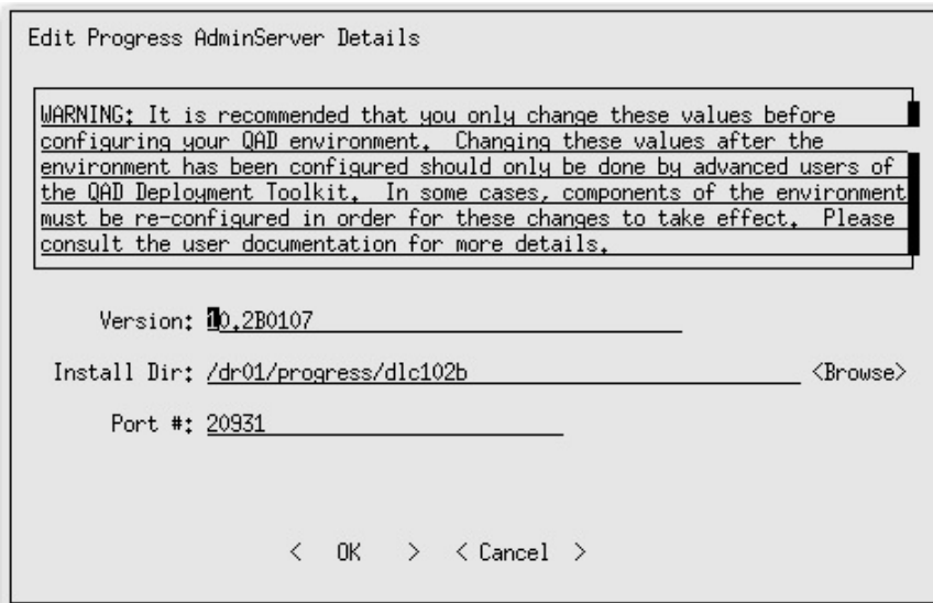
Fig. H.6 Edit System Details Screen
