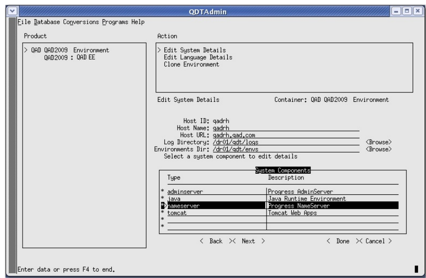
Fig. H.7 Specifying the Progress Name Server
