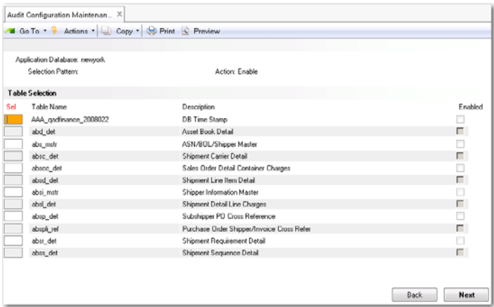
Fig. 8.5 Audit Configuration Maintenance Table Selection
