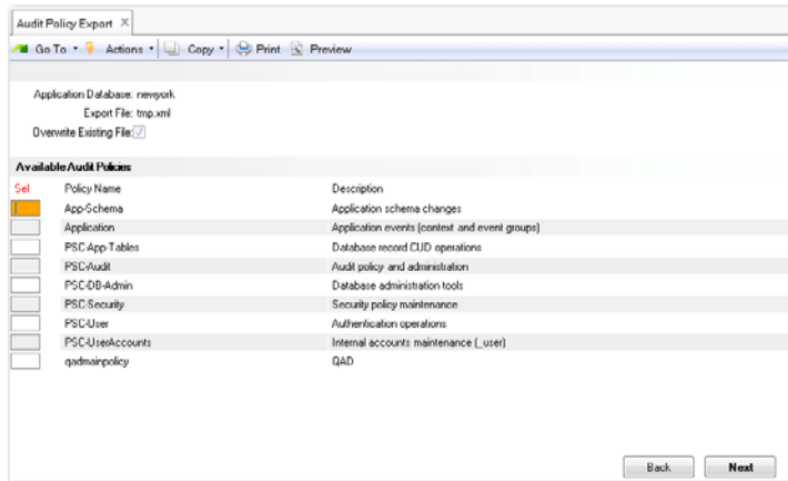
Fig. 8.13 Audit Policy Export (36.12.13.2)
