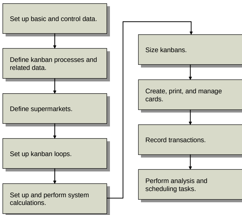
Fig. 3.3 Kanban Workflow
