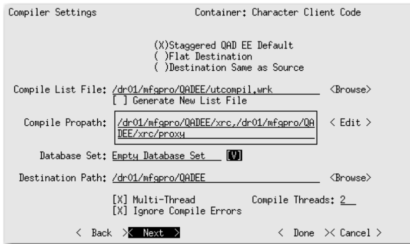
Fig. 3.10 Compiler Settings
