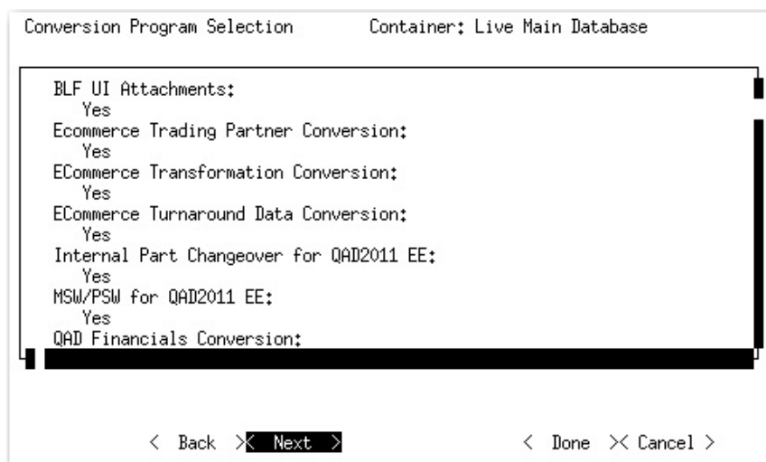
Fig. 5.7 Conversion Summary
