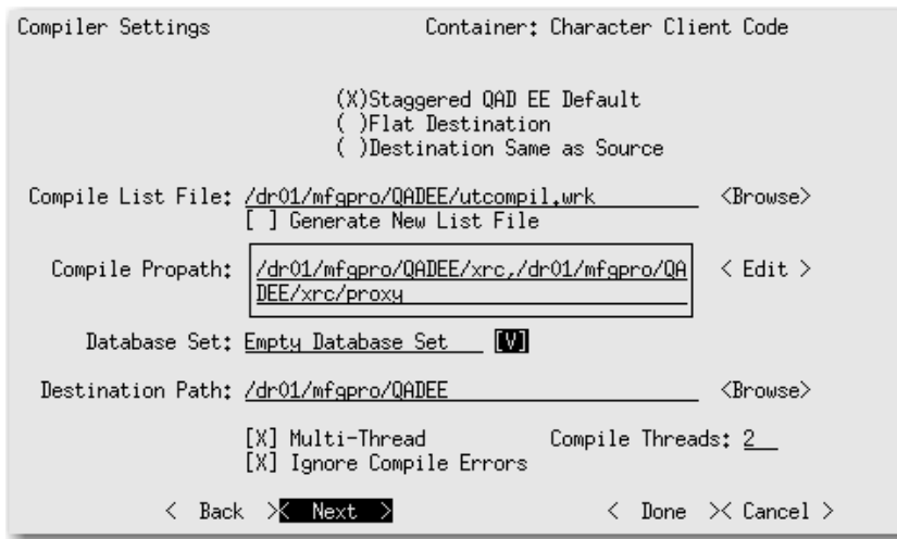
Fig. 3.10 Compiler Settings
