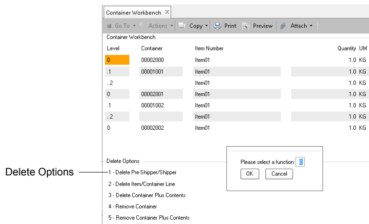
Fig. 6.46 Pre-Shipper/Shipper Workbench, Delete Options Pop-Up
