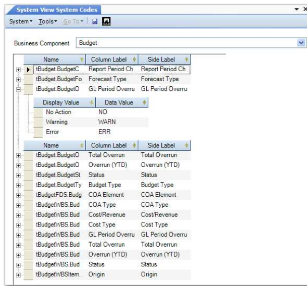
Fig. 6.4 System View System Codes (36.24.3.3)
