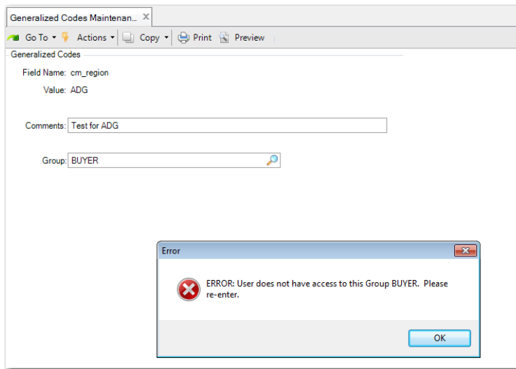
Fig. 2.6 Generalized Codes Maintenance (36.2.13)
