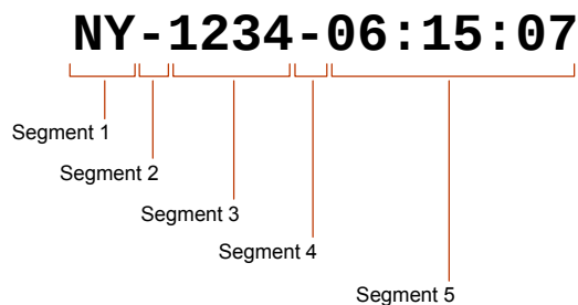
Fig. 2.8 Example Sequence Number
