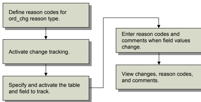
Fig. 2.18 Change Tracking Implementation Flow
