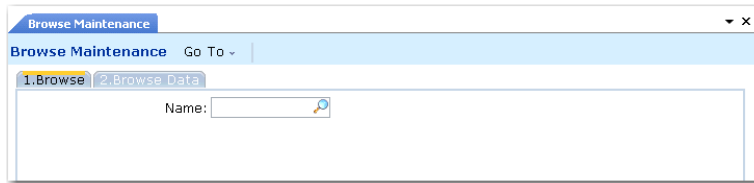
Fig. 3.16 Browse Maintenance (36.4.8.13)
