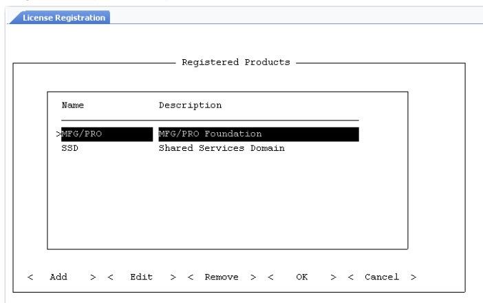
Fig. 8.4 License Registration (36.16.10.1)
