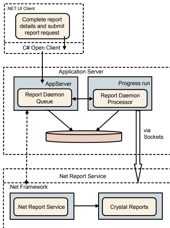
Fig. 5.12 Report Daemon Architecture
