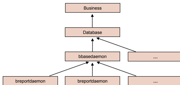
Fig. 10.2 Inheritance Structure
