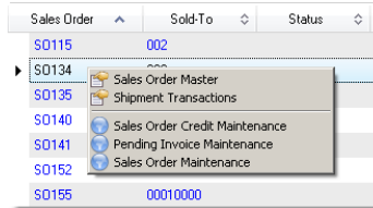
Fig. 4.54 Example of Browse Links
