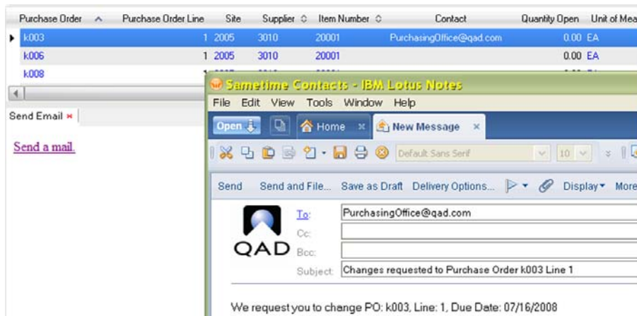
Fig. 4.60 Purchase Order Browse, Email Link
