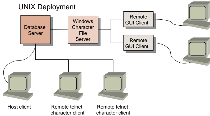
Fig. 1.1 Linux/UNIX Deployment
