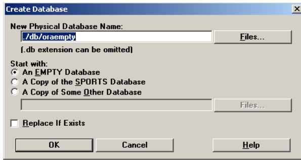
Fig. 3.13 Creating oraempty
