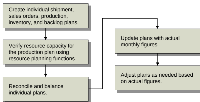
Fig. 15.1 Product Line Plan Process Flow
