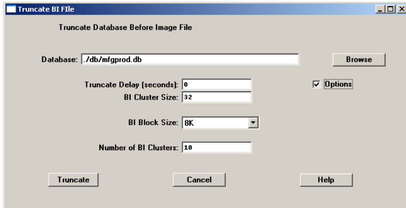
Fig. 10 Truncating mfgprod
