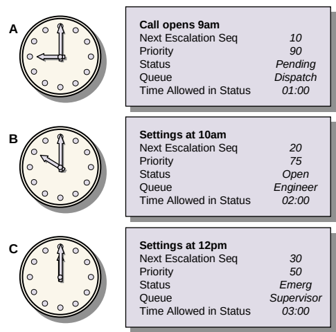
Fig. 15.1 Sample Call Escalation
