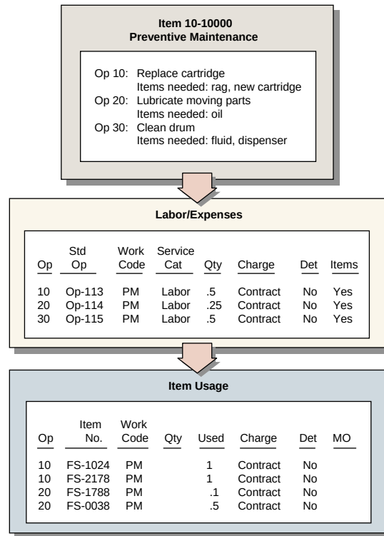
Fig. 13.4 Routing and BOMs Loaded into CAR
