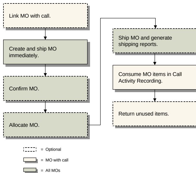
Fig. 19.3 Material Order Life Cycle
