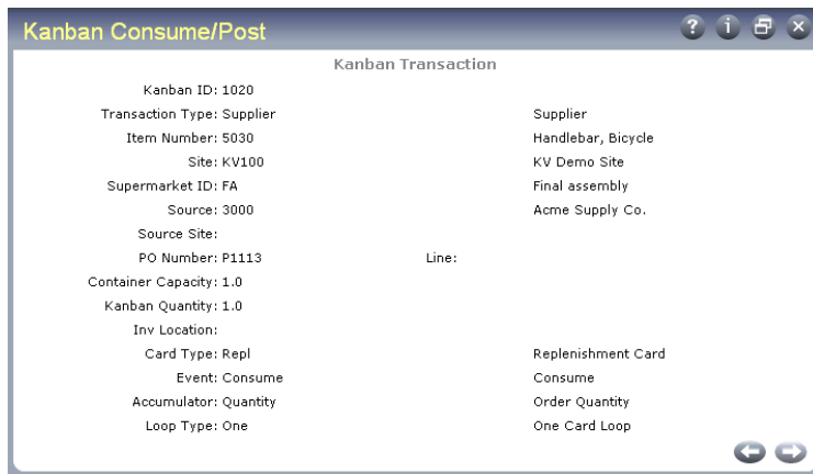
Fig. 1.57 Kanban Consume/Post, Kanban Transaction Summary Frame
