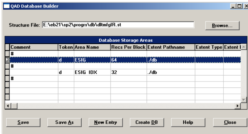
Fig. 1 Delta .st File Opened for Editing
