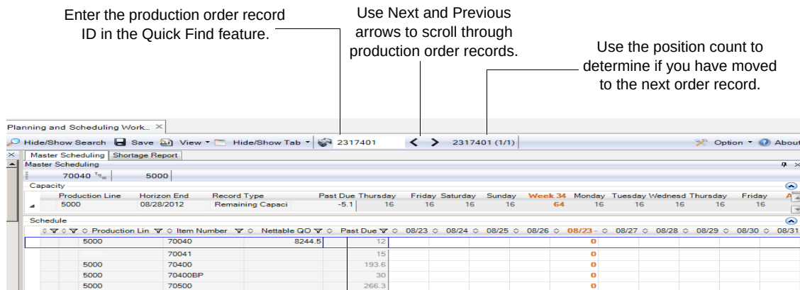
Fig. 2.1 Quick-Find Feature
