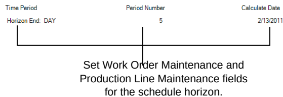
Fig. 2.11 Preferences
