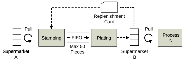
Fig. 1.1 Simplified Kanban Example
