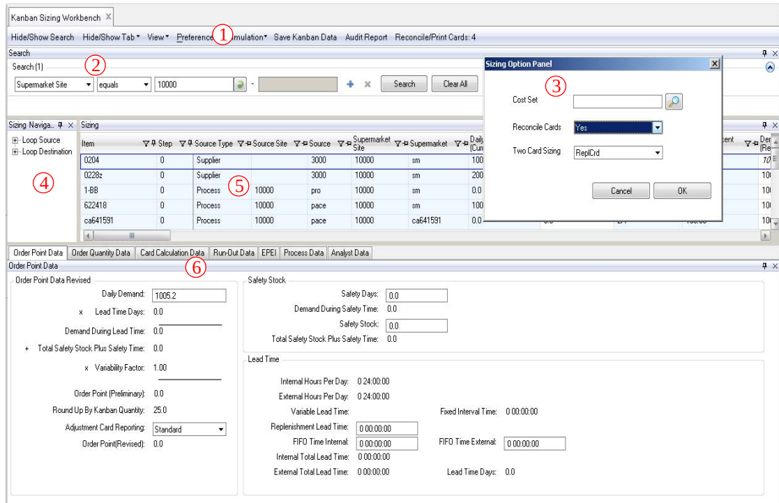
Fig. 1.32 Structure of Kanban Workbenches
