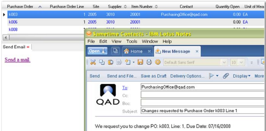
Fig. 4.59 Purchase Order Browse, Email Link
