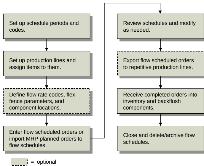
Fig. 8.1 Flow Scheduling Work Flow
