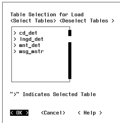
Fig. 5.30 Second Table Selection for Load Screen
