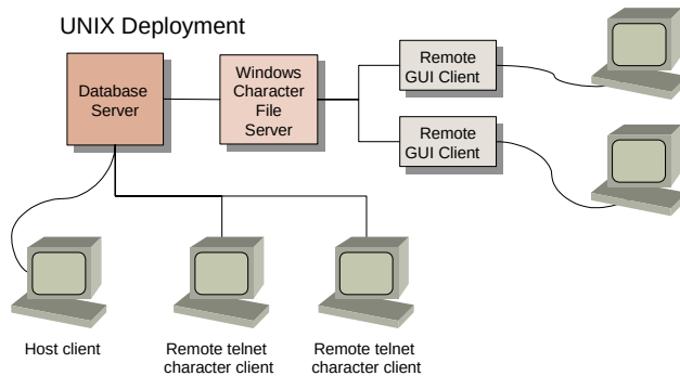
Fig. 1.1 UNIX Deployment
