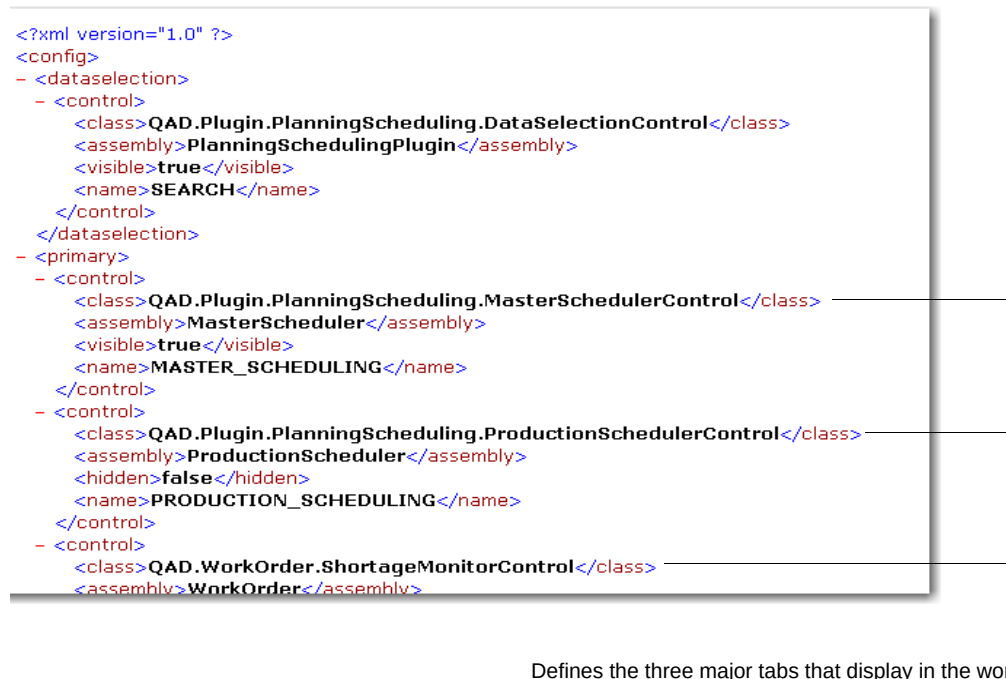
Fig. 4.5 ControlConfig.XML File
