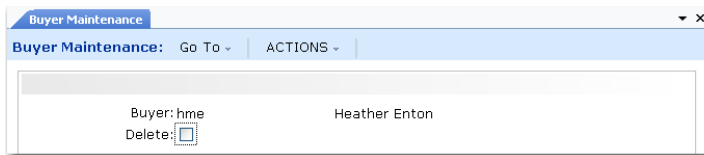
Fig. 2.10 Buyer Maintenance (5.2.1.20)
