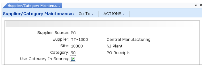
Fig. 5.11 Supplier/Category Maintenance (5.15.3)
