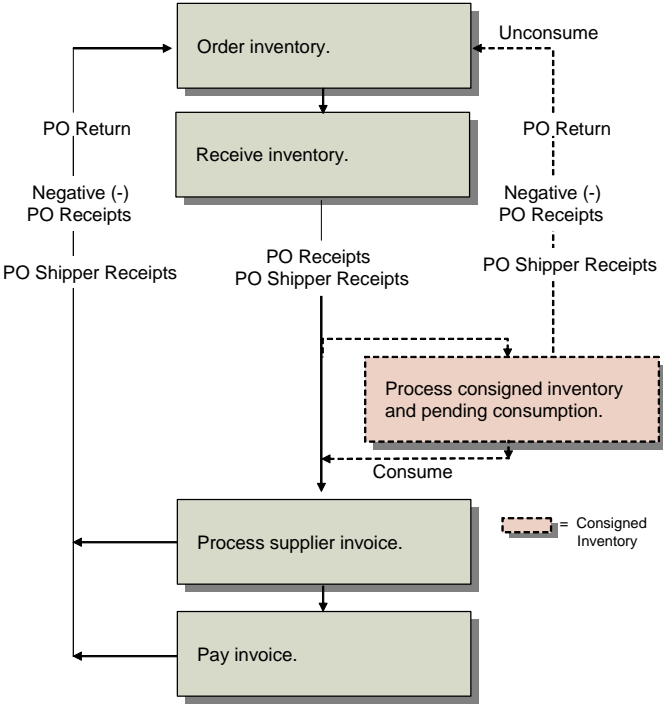
Fig. 4.2 Consignment Overview
