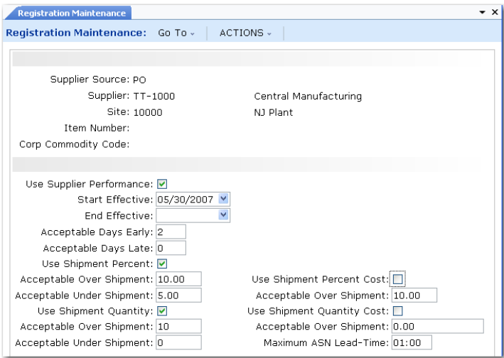
Fig. 5.10 Registration Maintenance (5.15.10)
