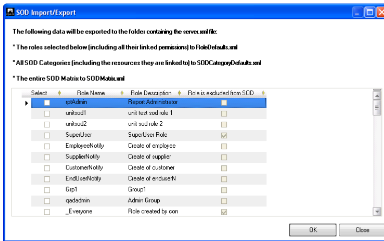
Fig. 5.35 XML Export Dialog
