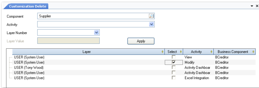
Fig. 12.20 Customization Delete
