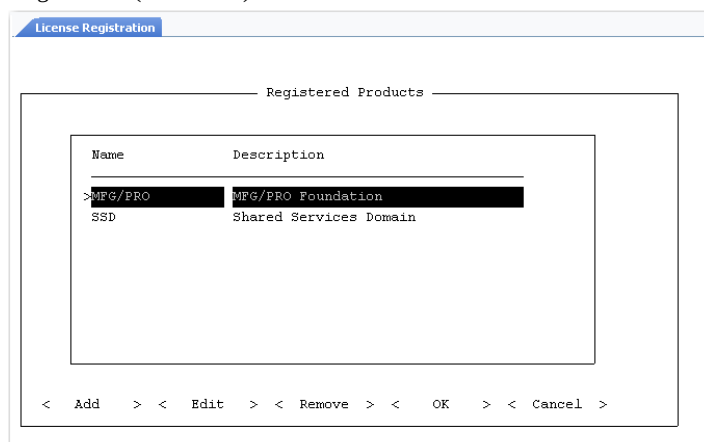
Fig. 8.4 License Registration (36.16.10.1)
