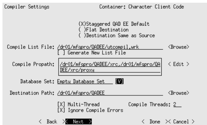
Fig. 3.9 Compiler Settings
