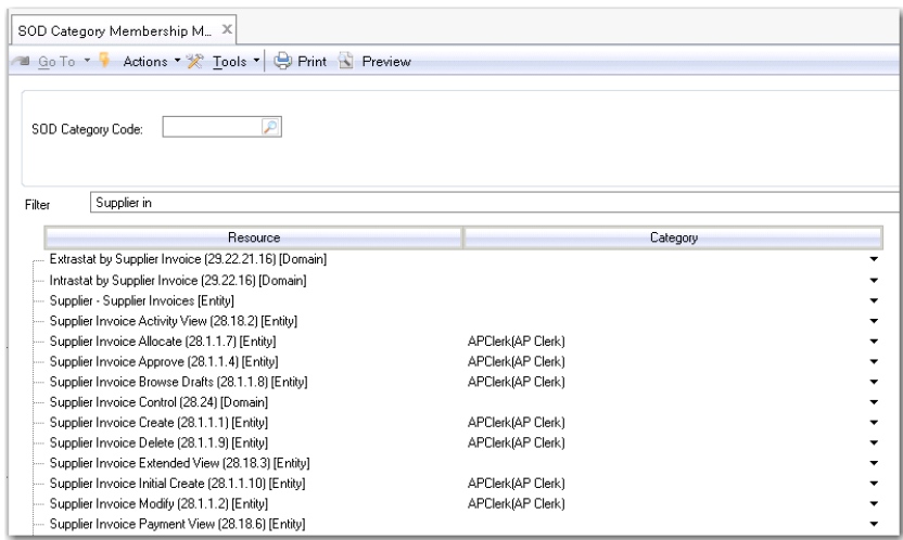
Fig. 5.13 SOD Category Membership Maintain, Filtering
