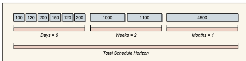
Fig. 4.9 Schedule Bucketing
