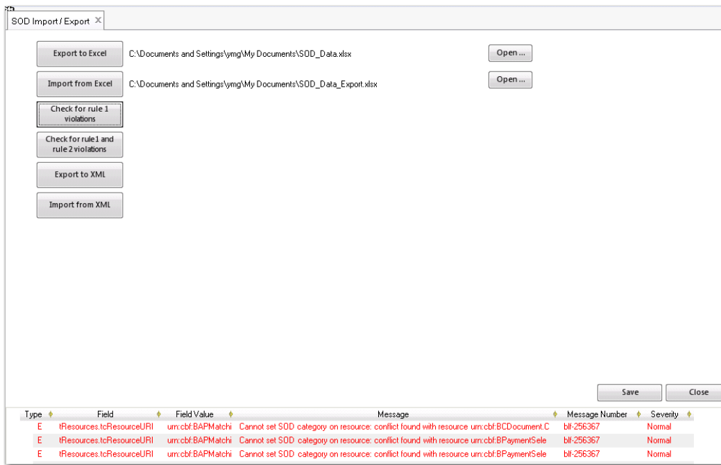
Fig. 5.32 Violation Errors
