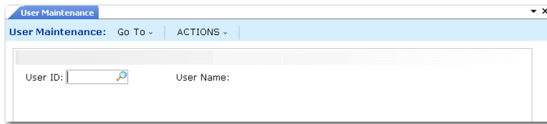
Fig. 4.3 User Maintenance (36.3.1)
