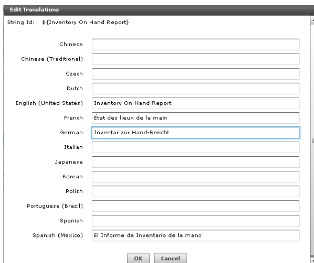
Fig. 2.39 Edit Translation
