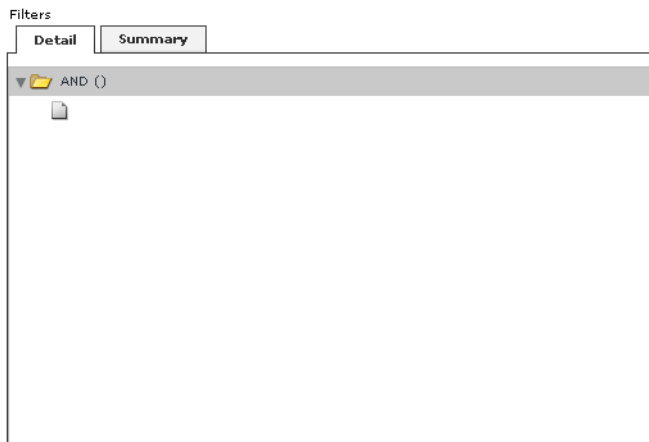
Fig. 3.10 Filters Pane
