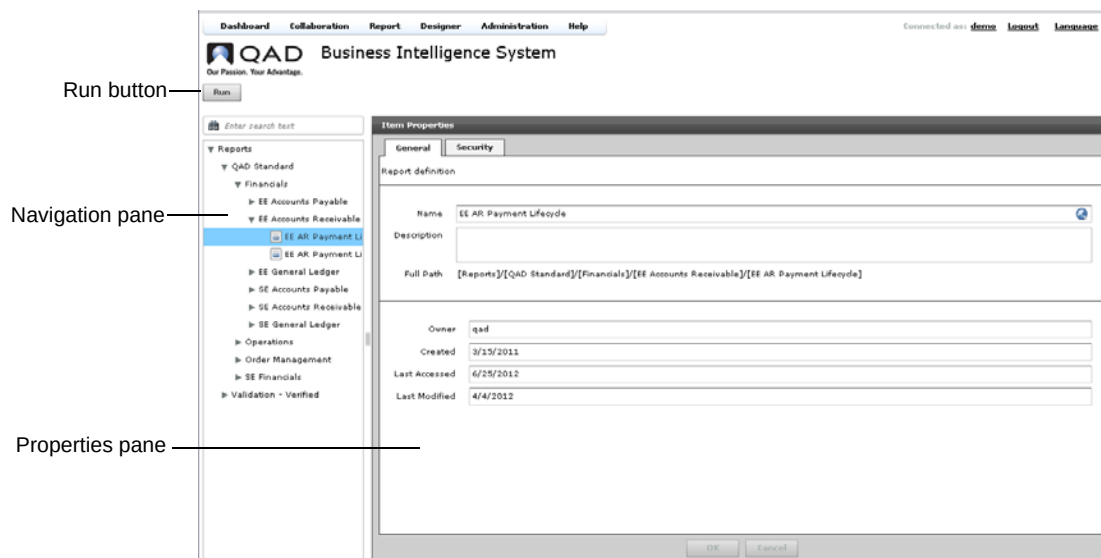
Fig. 2.19 Report Home
