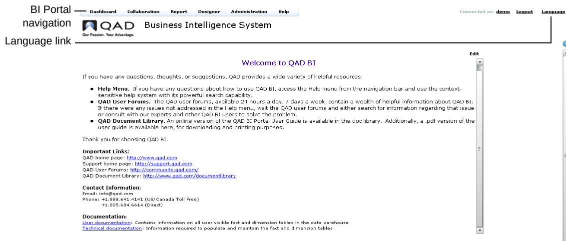
Fig. 2.4 Welcome Screen
