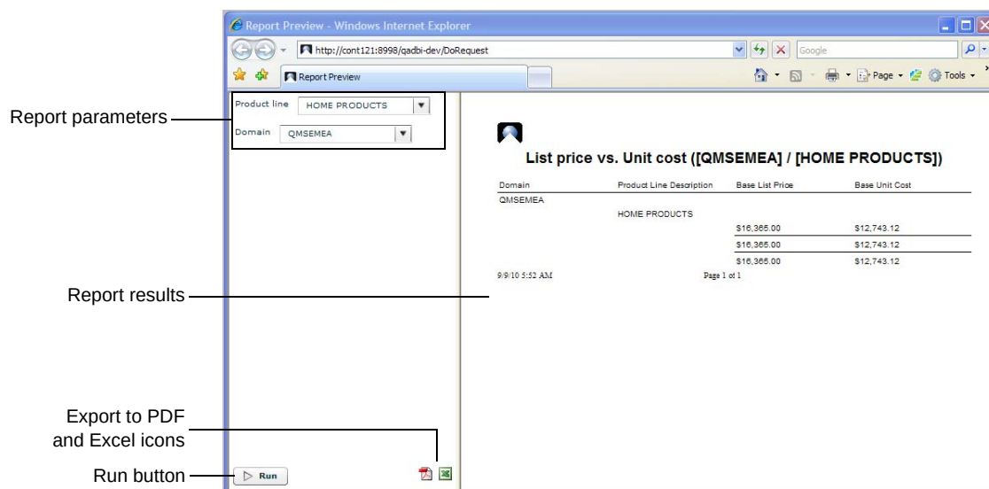
Fig. 2.20 Report Preview
