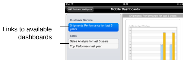
Fig. 2.31 Mobile Dashboards
