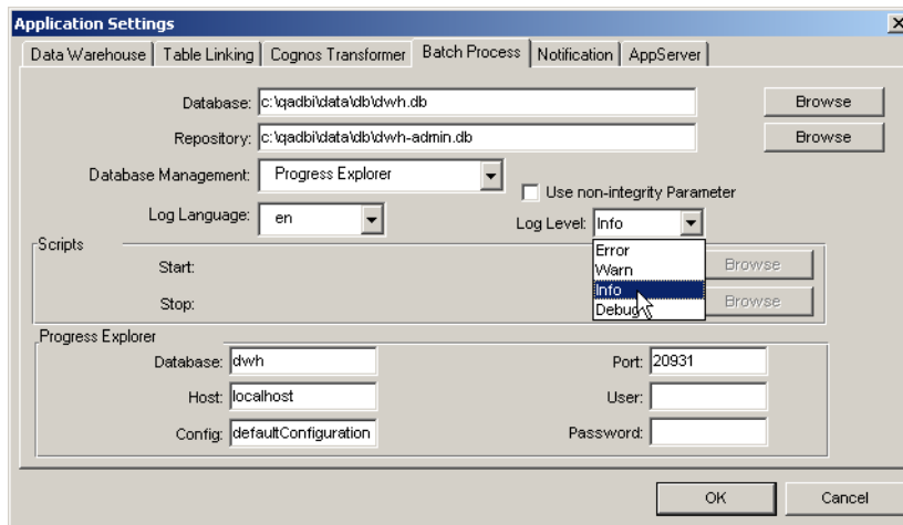
Fig. 6.49 Application Settings, Batch Process Tab
