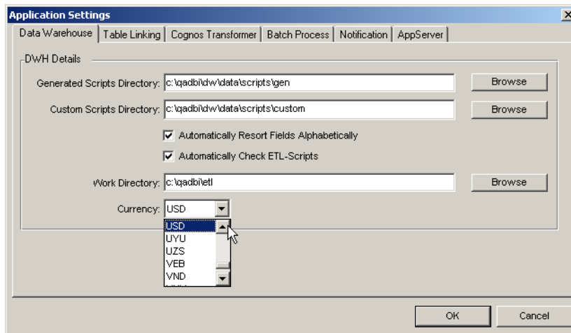
Fig. 7.9 Setting the Data Warehouse Currency
