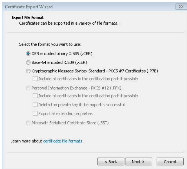
Fig. 8.5 Certificate Export Wizard Dialog Box - Export File Format
